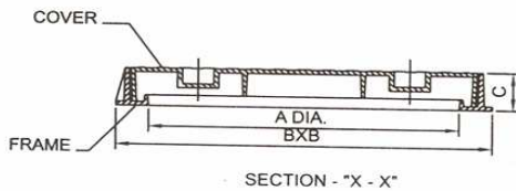
CIRCULAR COVER WITH SQUARE FRAME
