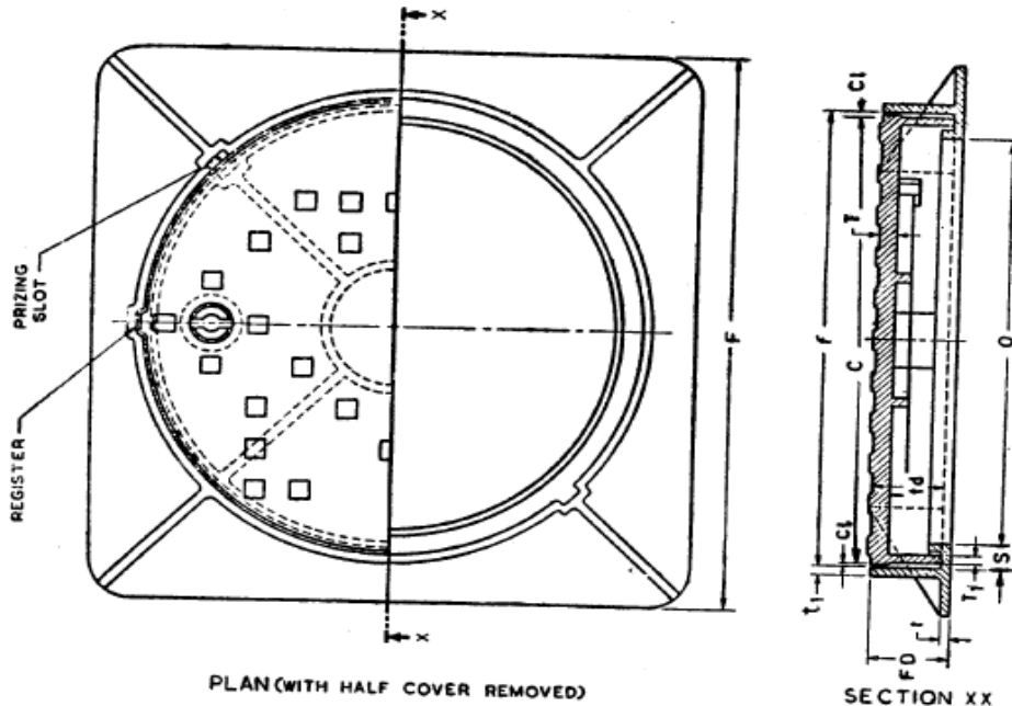
FIG. 6 HEAVY-DUTY AND MEDIUM-DUTY CIRCULAR COVER AND FRAME
