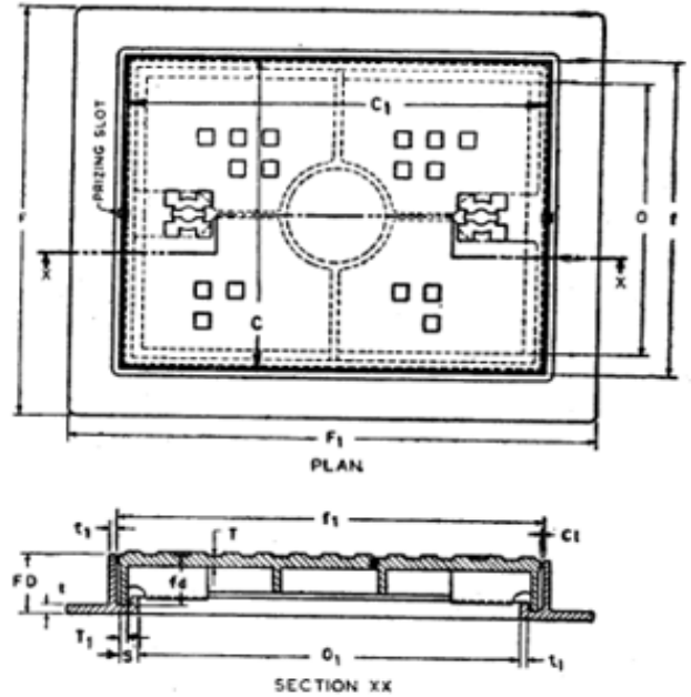
FIG. 7 TYPICAL MD/HD/EHD RECTANGULAR MANHOLE COVER AND FRAME
