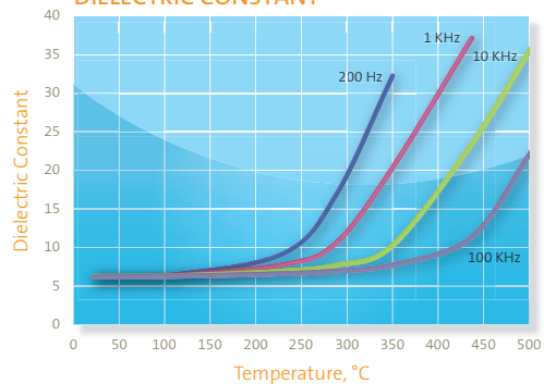
DIELECTRIC CONSTANT
