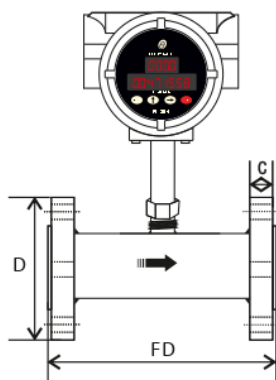
Fig. 1 Front View
