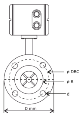
Fig. 2 Side View
