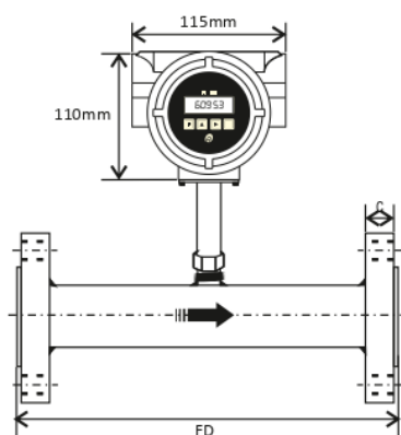
Fig. 1 Front View
