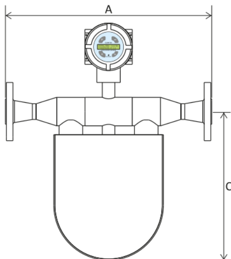
Fig. 1 Front View
