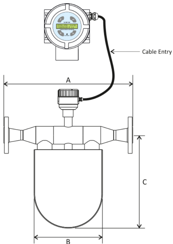
Fig. 3 Front View
