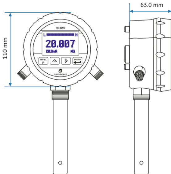
Fig. 1 Front View
