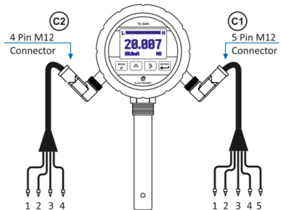
Fig. 3 Front View
