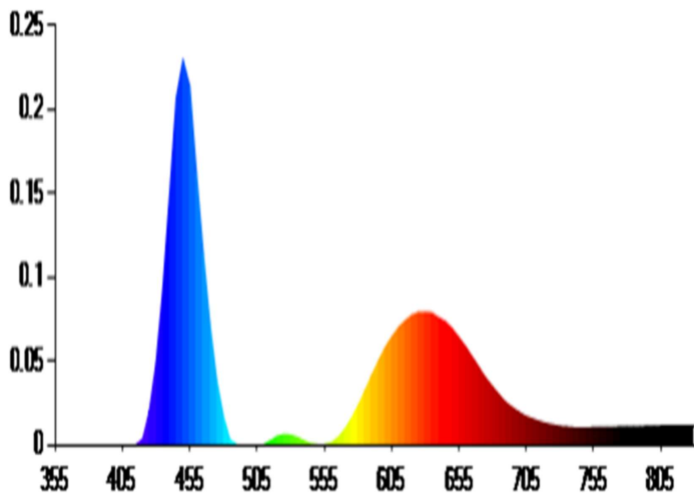
Spectral Power Distribution
