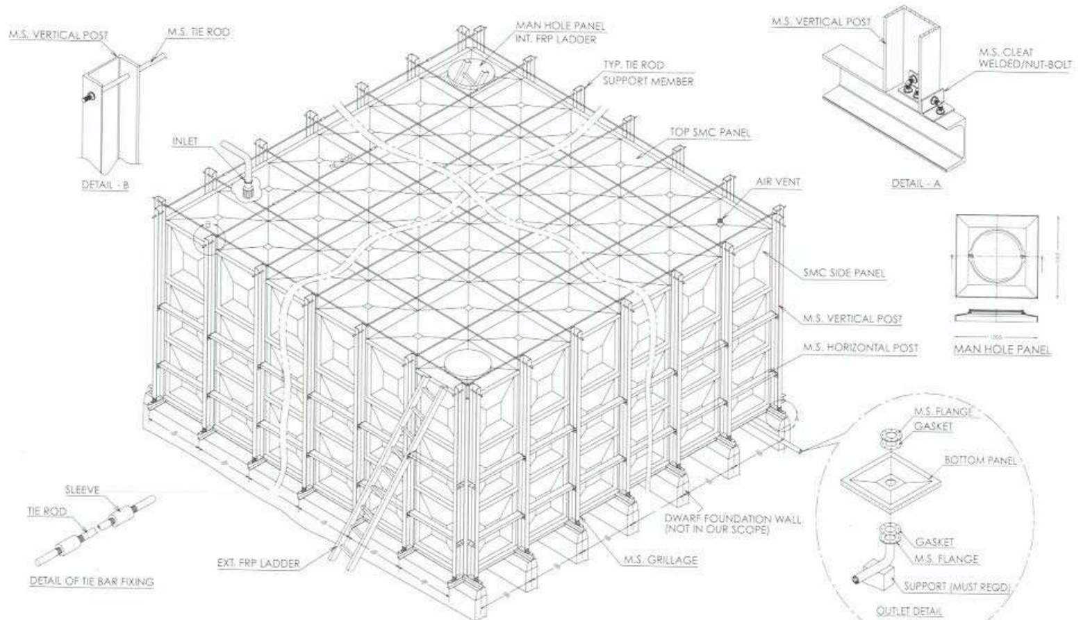
General arrangement drawing for ground level - SMC Panel tank 3m height
