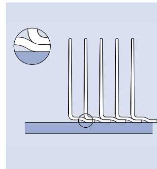
LL Fin (Overlapped L Fin)
