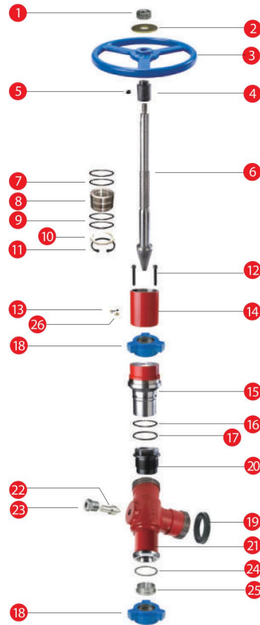
3" Adjustable Choke Valve Repair Kit
