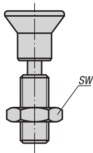
Form H with locknut
