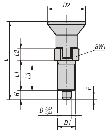
Form CP lockout type without locknut
