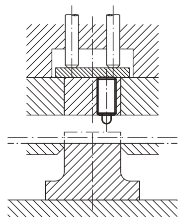
Spring plunger sectional view
