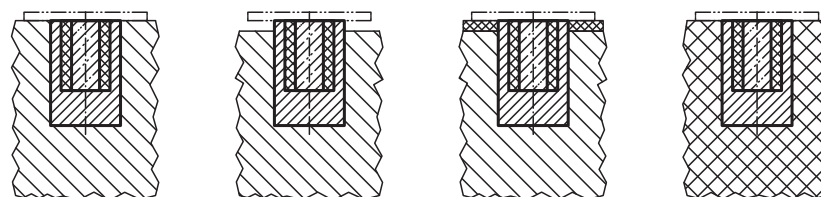
Mounting instructions for shielded pot magnets without pins
