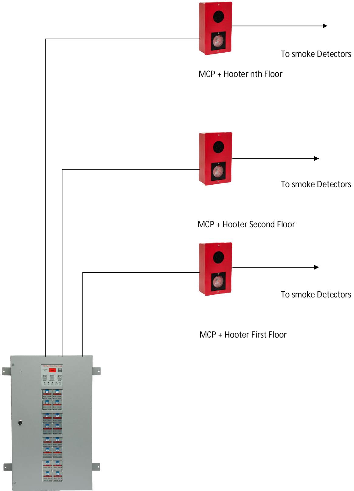
WIRING DIAGRAM OF PUBLIC ADDRESSABLE PANEL Je190
