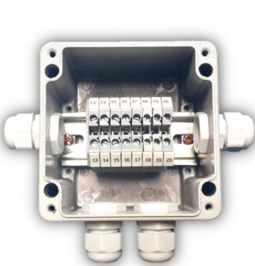
8 Terminal Junction Box
